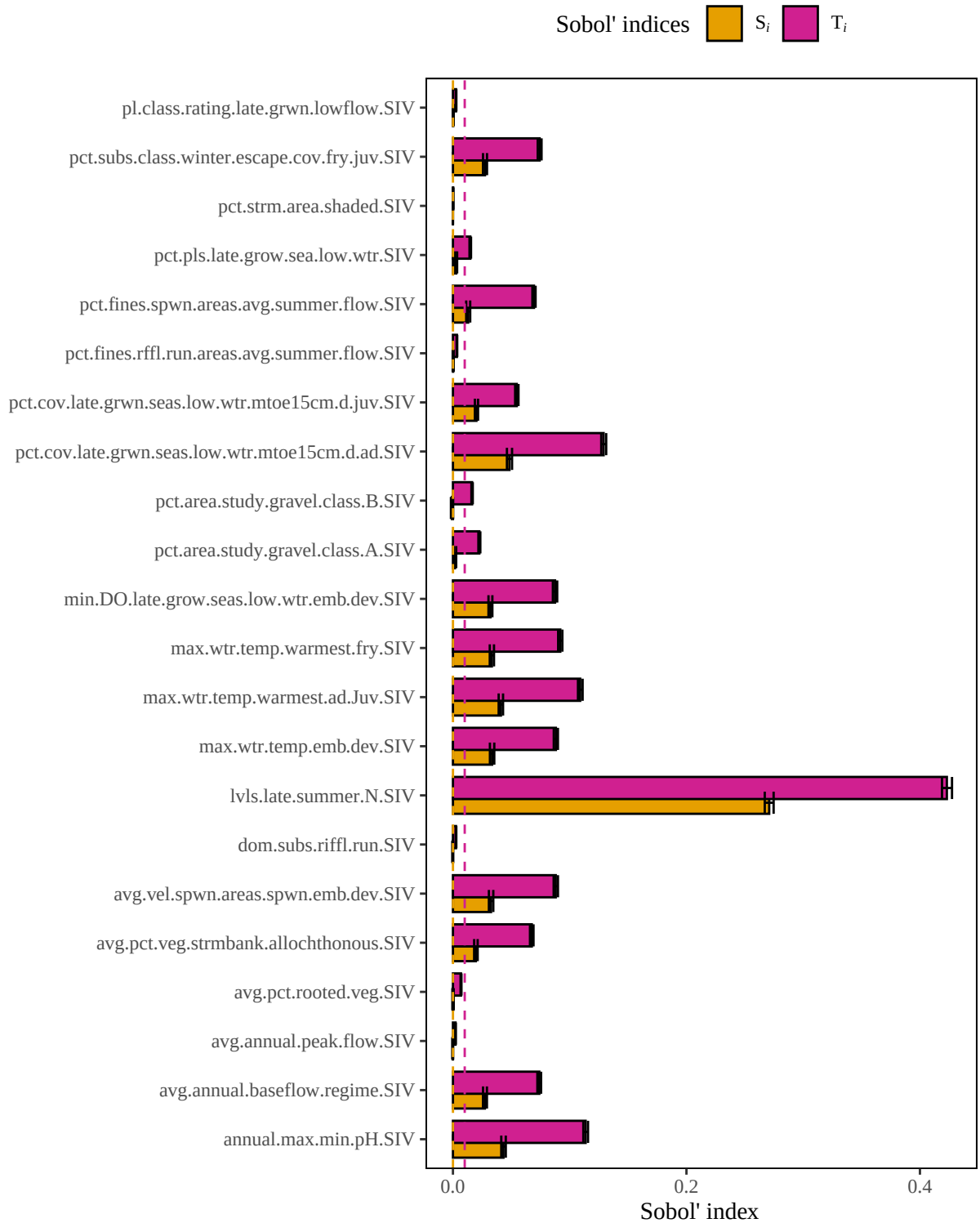
Figure 3. Results of a sensitivity analysis for the brownt troutLimitMt10C model based on the original limiting factor model outlined in Raleigh et al. (1986). Dashed lines represent baseline numerical approximation error for S_i and T_i ( i.e. , dummy variables).
