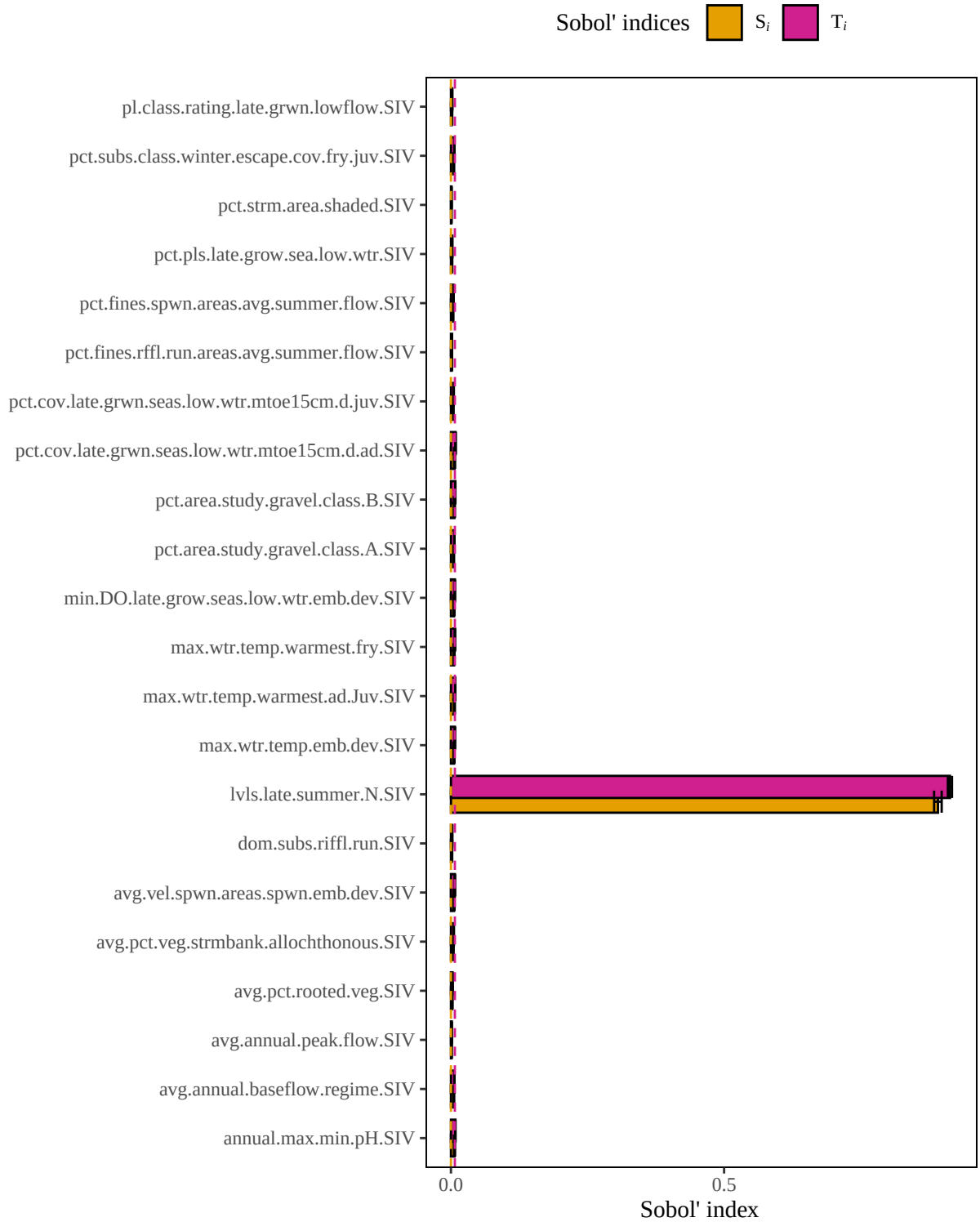
Figure 5. Results of a sensitivity analysis for the brownt troutLimitMt10C model based on a geometric mean structure. Dashed lines represent baseline numerical approximation error for S_i and T_i ( i.e. , dummy variables).
