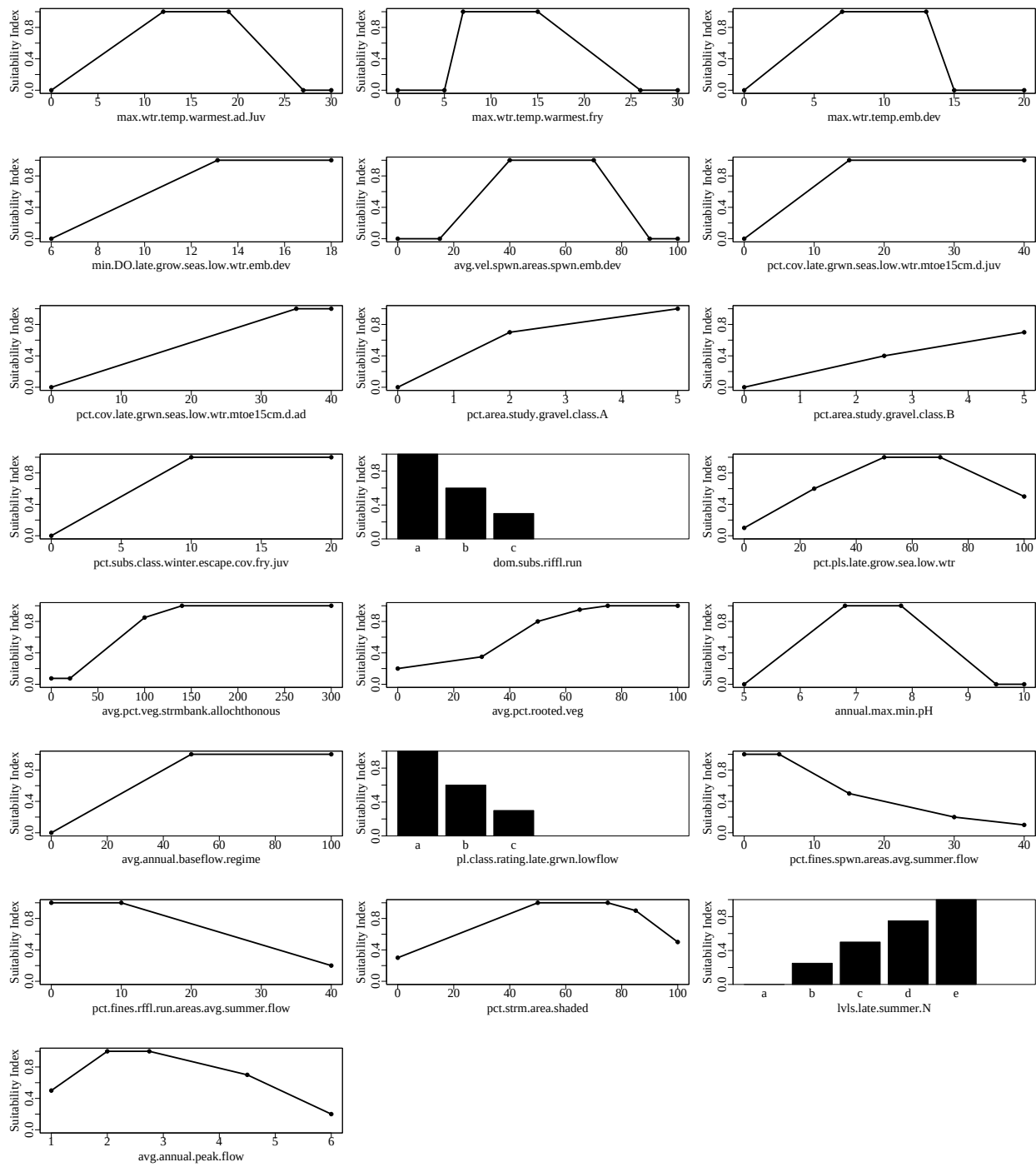
Figure 1. Suitability index graphs for variables included in the browntrountLimitMt10C model in ecorest.
